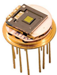
MEMS based micro spectrometer module and spectral response (from InfraTec)
